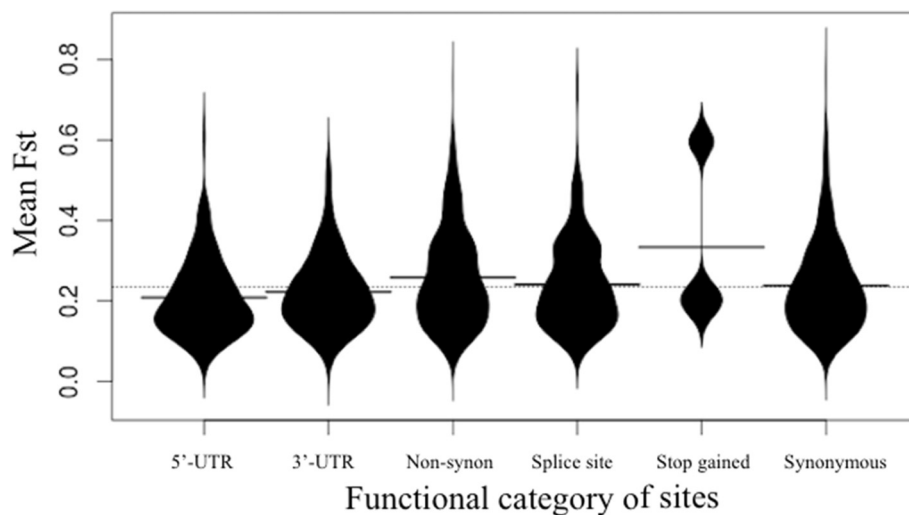
Fig. 3 Distribution of mean Fst in 50kb windows centered around putatively functional sites. Polymorphic sites with F_{st} \geq 0.75 between dogs and wolves were classified according to their putative function. For each putatively functional site the mean Fst was calculated in a 50kb window centered on the site. A violin plot shows the distribution of mean Fst values for each category of functional site (5'-UTR, 3'-UTR, non-synonymous, splice site, stop gained, synonymous). Synonymous mutations were included as a category to show the expectation in the absence of positive selection
