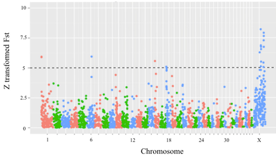
Fig. 1 Genome-wide scan for selective sweeps. Z-transformed mean Fst calculated in 500kb genomic windows across the autosomes and X chromosome between dogs and wolves. Each point represents a 500kb window. A dashed horizontal line represents our threshold for identifying putatively selected regions ( >5 Z(Fst)). 18 windows exceed this threshold and are considered as putative selective sweeps
