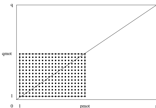
FIGURE 1. Lattice points
