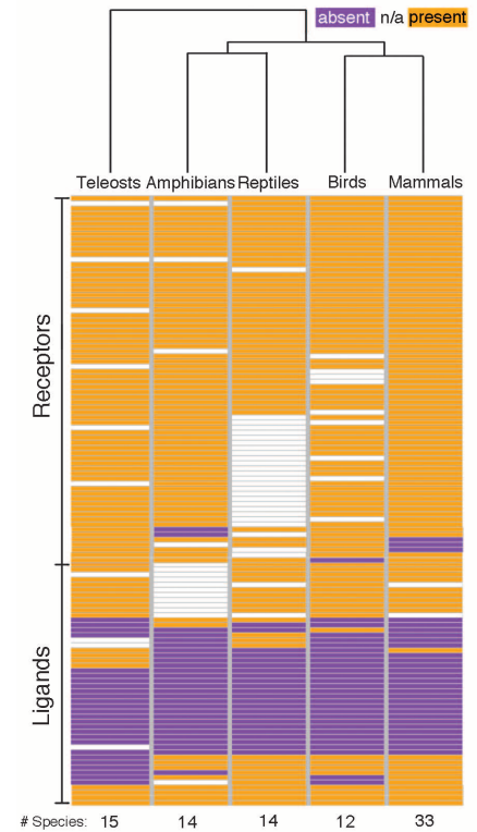
Fig. 2. Analysis of vertebrate patterns in brain neurochemistry. Overall patterns in neurochemistry in the social decision-making network are shown across vertebrates. Data for each vertebrate lineage are represented in the columns, and each row represents one gene in one brain region that is either present (orange) or absent (purple). White indicates that no data are available (n/a). The number of species in each vertebrate lineage represented in the analysis is shown at the bottom of each column. The dendrogram (top) is the result of unsupervised hierarchical clustering of the vertebrate neurochemical patterns.
